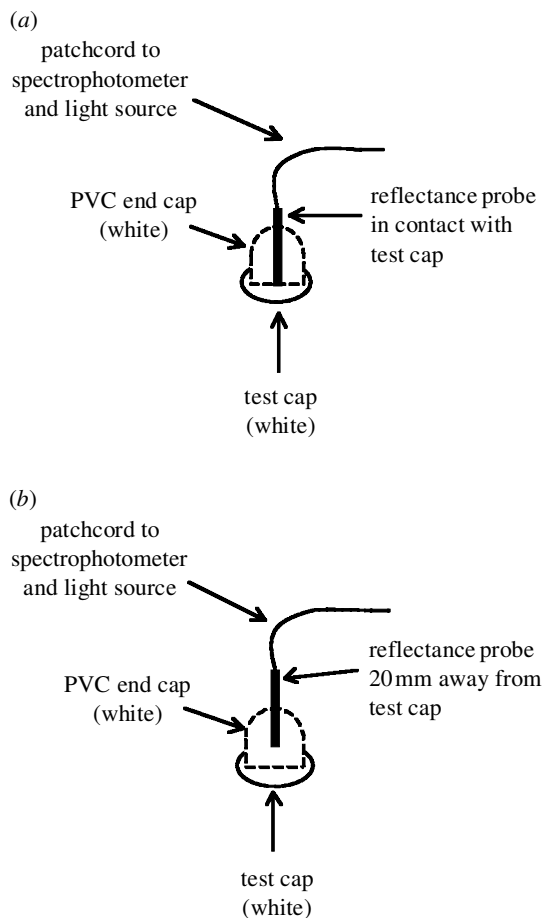
Figure 2. Schematic diagram of apparatus used to measure light transmission through the water. A white PVC end cap sits on a white test cap. The end cap is opaque and does not allow any sunlight to enter the chamber. The dashed line denotes that the schematic diagram is showing what happens inside the chamber. The reflectance probe fits snugly through a small hole in the top of the end cap. (a) Reflectance probe in contact with test cap. Light emerges out of the probe, is reflected off the test cap, and is then detected by the sensors in the probe. This determines the maximum amount of light detectable. (b) Reflectance probe 20 mm away from the test cap. Light emerges out of the probe, is transmitted through the water, bounces off the test cap and the inside of the end cap, and then is detected by the sensors in the probe. The proportion of light transmitted through the water can be calculated by comparing the amount of light detected here with the maximum amount of light possible and the minimum amount of light possible (complete darkness).
